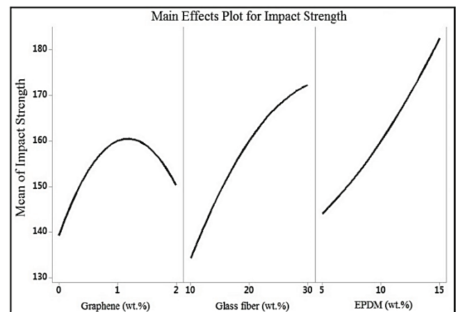
Figure 1 Main effects plot for impact strength
